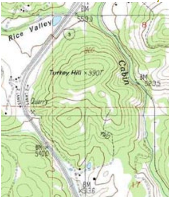
USGS 1:24:000 scale topographic maps are very useful for describing the positions of natural and man-made features around your property.
